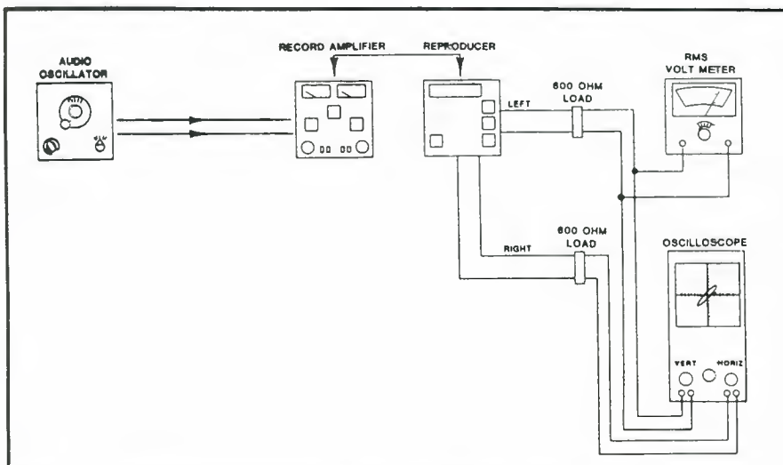
Figure 1. A typical test setup for checking the performance of a record/play tape cartridge system. Closely follow the manufacturer's recommendations on mechanical and electrical alignment for best results. (Courtesy ITC/3M.)
