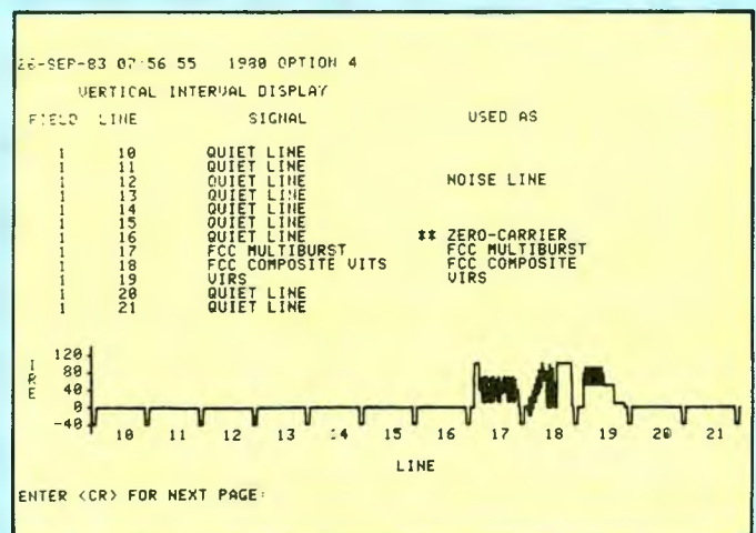
Figure 2. Vertical interval line assignments and display.
