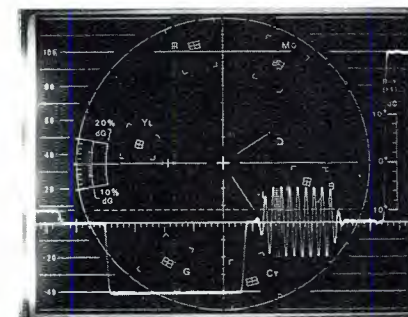
Figure 1. The horizontal blanking interval, shown in waveform mode in 1 s/div. sweep speed.
